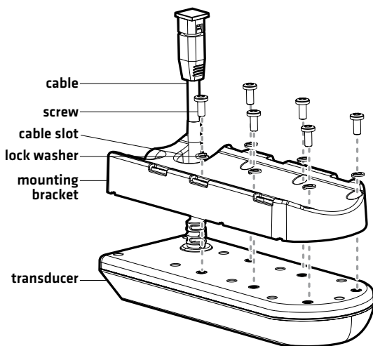
Installing the Mounting Bracket
