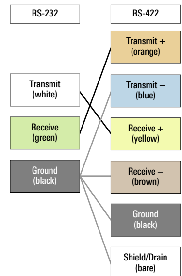
Chart 4 (Optional Wiring) RS-232 to RS-422
