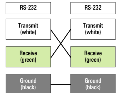
Chart 3 (Optional Wiring) RS-232 to RS-232
