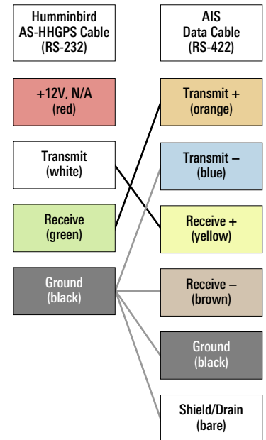
Chart 2 (Optional Wiring) RS-232 AS-HHGPS to RS-422 AIS
