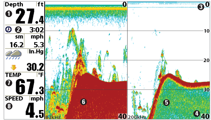
Split Sonar View (858c, 958c, 898c SI, and 998c SI)
