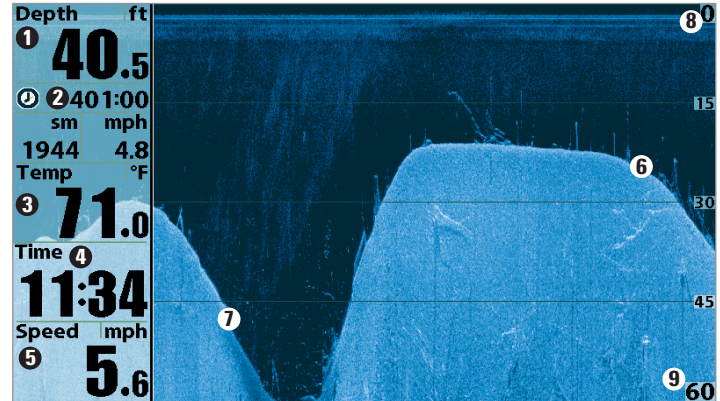
Down Imaging™ View
