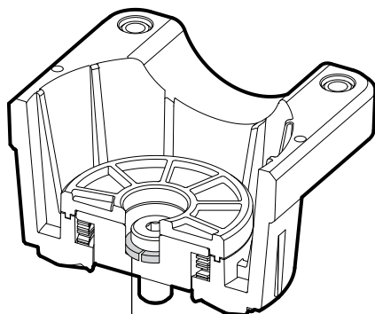
fully compressed lock washer
