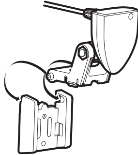
Inserting the Pivot Arm Assembly into the Mounting Bracket
