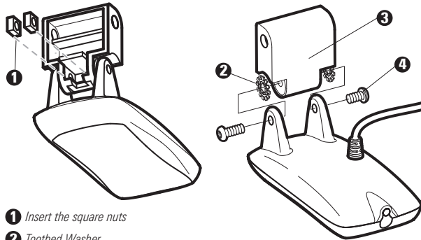
Attach the Pivot
